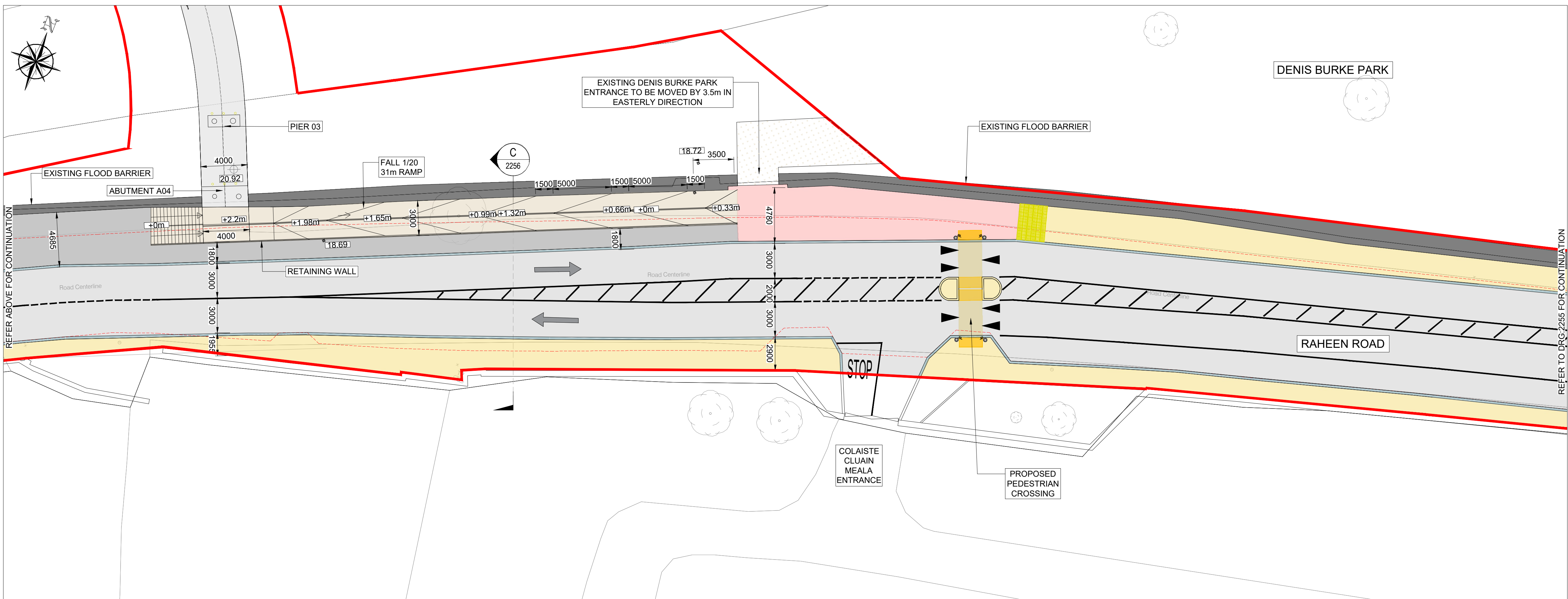
PLAN 5 SCALE 1:200
